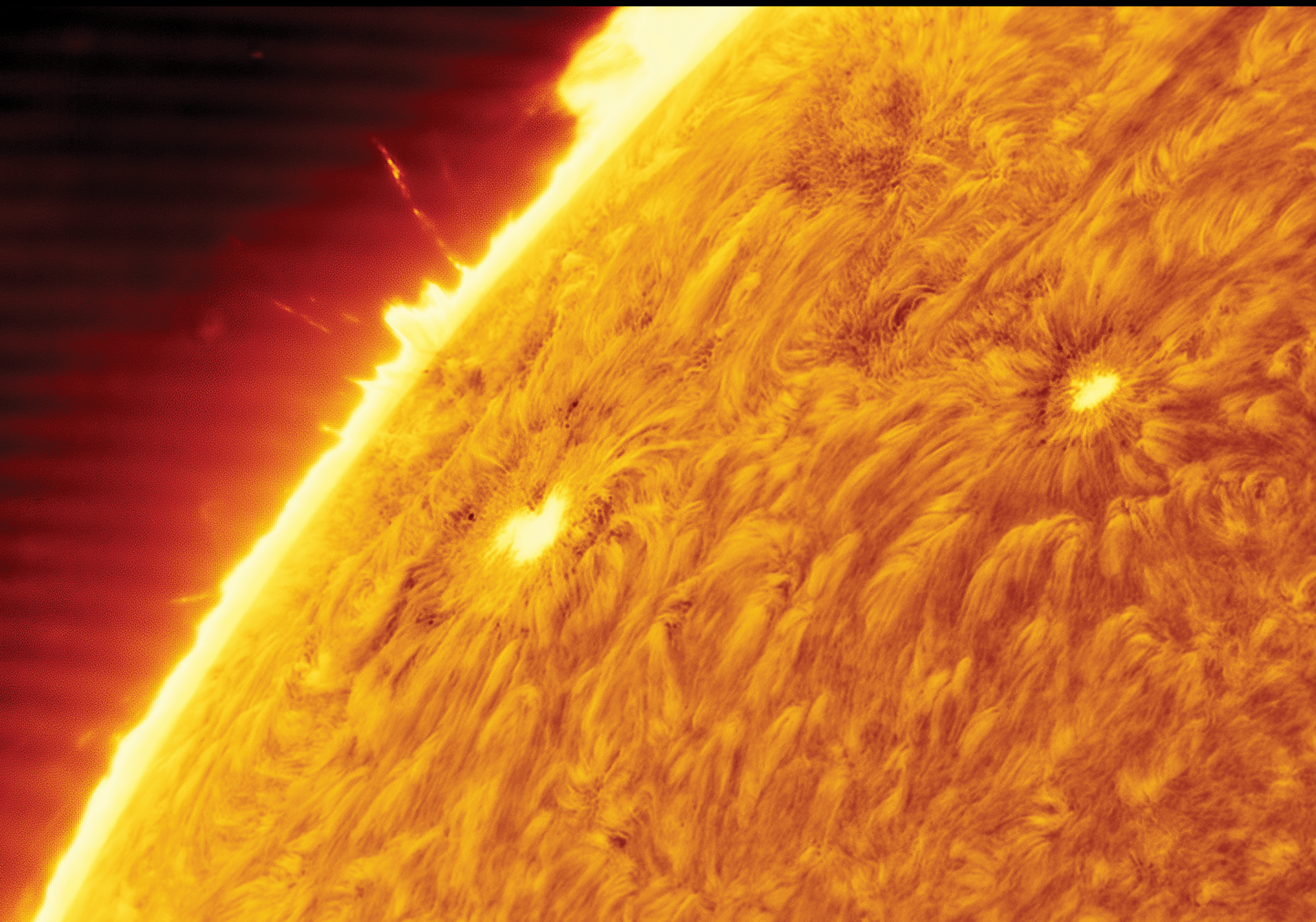
A small part of the Sun's surface on which two Sun spots are seen. The larger one is three times the size of the Earth. The temperature of the Sun's surface is about 6000 degrees while in its center the temperature reaches about 15.7 million degrees. Photographed by David Dayag through a 15.2 cm telescope and an H \alpha filter.
